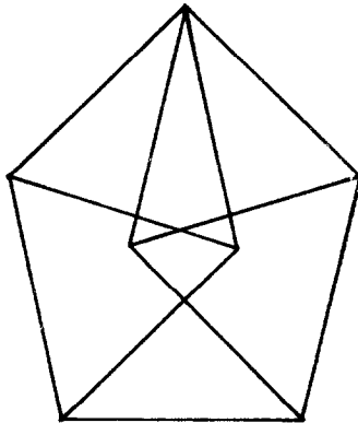
FIG. 1. All edges have length d .
