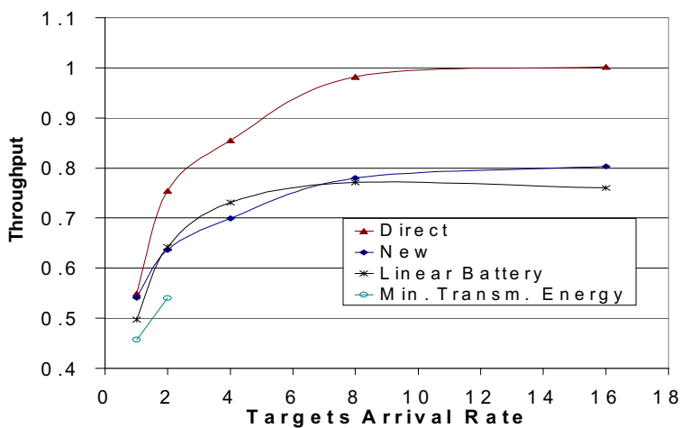
Fig. 10: Comparison between different routing algorithms (Network Throughput)
