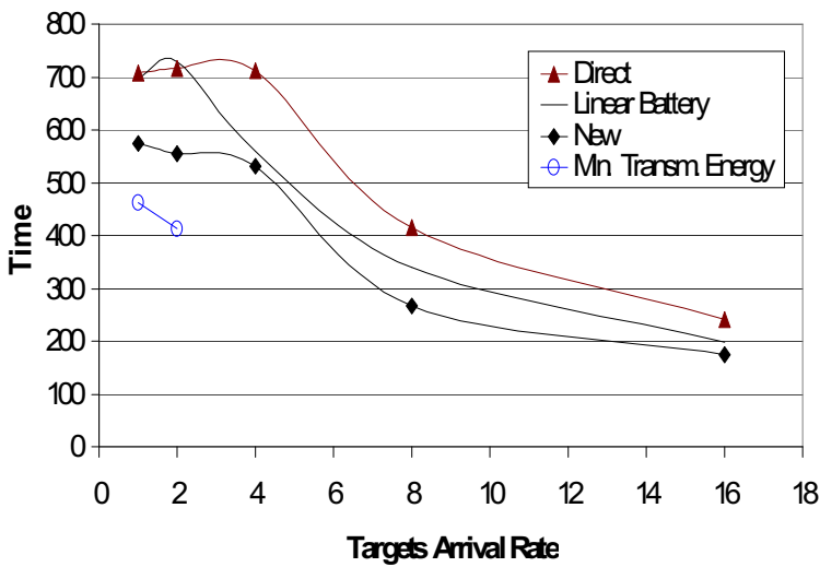
Fig. 8: Comparison between different routing algorithms (Standard deviation of nodes lifetime)
