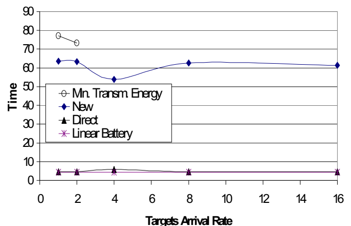
Fig. 5: Comparison between different routing algorithms (Time to network partition)
