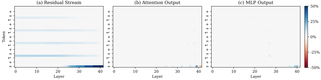
Figure 20: Activation Patching By Token.
