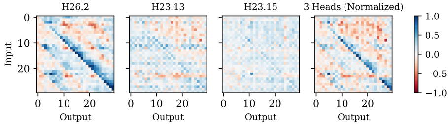
Figure 28: Individual and Overall Effect of FI Heads in Off-by- k Addition, k = 1 , Llama-3 (8B). While Llama-3 (8B) uses [0,999] tokenization, we visualize results in the range of [0,29] for readability. H26.2 promotes x + 1 and sometimes x + 2 ; H23.13 and H23.15 promotes x - 1 and x + 1 . They collectively contribute to promoting x + 1 as the output.
