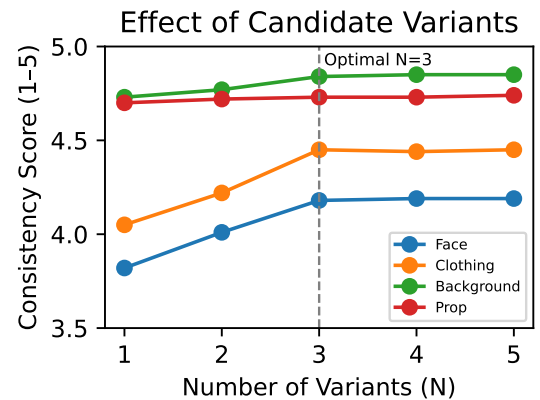
Figure 5: Effect of generating N candidates on the ContinuityEval metrics.
