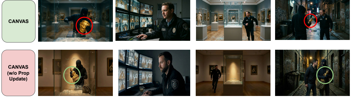
Figure 6: Qualitative Ablation showing the importance of Prop-State Tracking in CANVAS.
