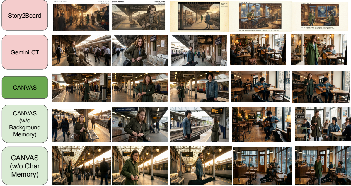
Figure 4: Qualitative Examples of Train Story from HardContinuityBench along with ablation showing the importance of Background and Character Memory Update. CANVAS best preserves character and scene continuity across shots; removing either background or character memory causes clear consistency failures, highlighting the importance of both memory components.
