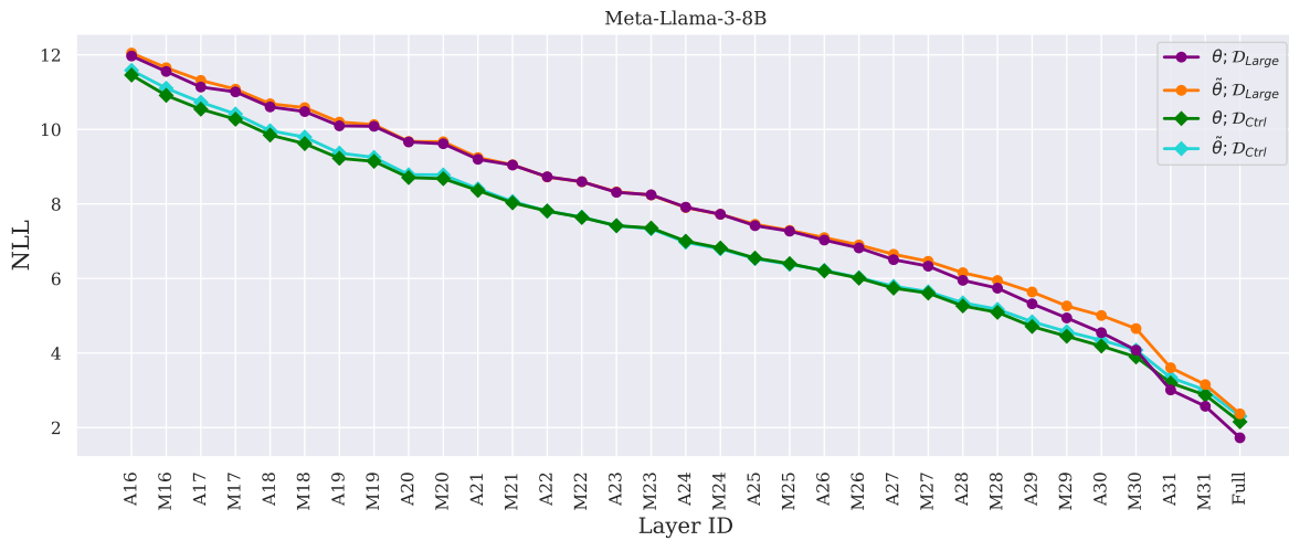
Figure 13: Early Exiting results on Llama3-8B. We decode the inputs to z^{(l)} (A#) and r^{(l)} (M#) across layers.
