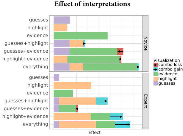
Figure 2: Coefficients of the linear regression showing the effects of interpretations, for novices (above) and experts (below). Higher value means an interpretation improves player accuracy. In addition to the individual interpretations, combo gain and combo loss capture the additional effect of combining multiple interpretations. Highlight and Evidence are effective for both novices and experts; combining leads to more positive effect for experts than novices, potentially because experts can process more information in limited time.
