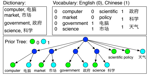
Figure 1: An example of constructing a prior tree from a bilingual dictionary: word pairs with the same meaning but in different languages are concepts; we create a common parent node to group words in a concept, and then connect to the root; uncorrelated words are connected to the root directly. Each topic uses this tree structure as a prior.
