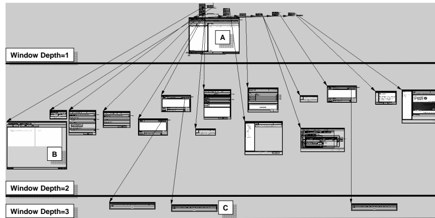
Fig. 13. An Example GUI Windows Hierarchy.
