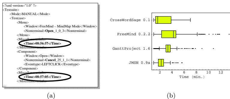
Fig. 6. (a) Time-stamps in a Test Case and (b) Time Taken to Record Each Test Case.
