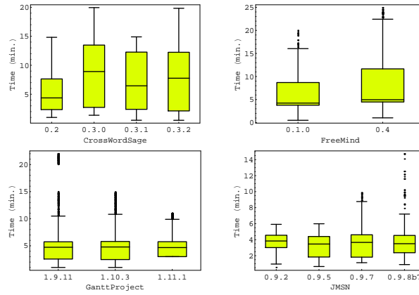
Fig. 16. Time Taken to Record Each Supplemental Test Case.
