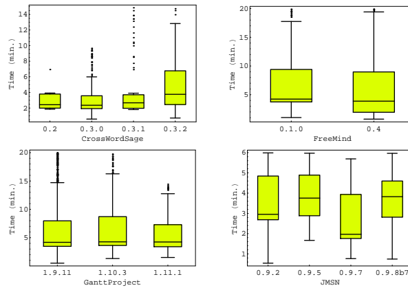
Fig. 7. Time Taken to Record Each Additional Test Case.
