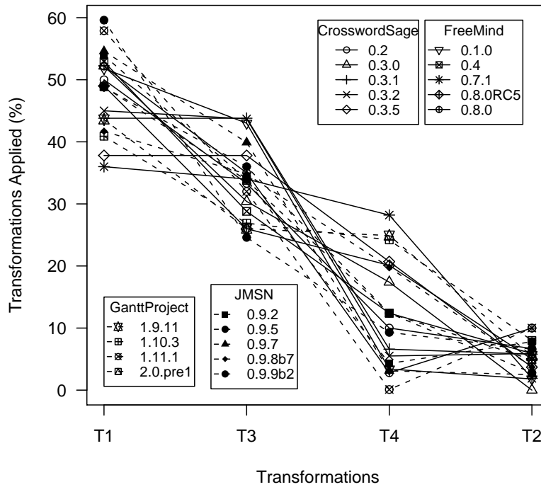
Fig. 8. Transformation Type and Percentage Applied on Each Application Version.
