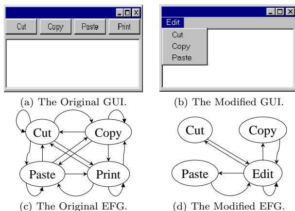
Fig. 1. A Regression Testing Example.
