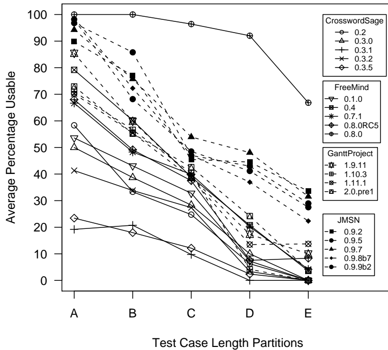
Fig. 11. Average Percentage of Usable Test Cases Partitioned by Length.
