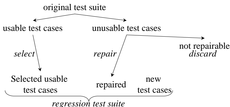
Fig. 2. The New Regression Testing Method.
