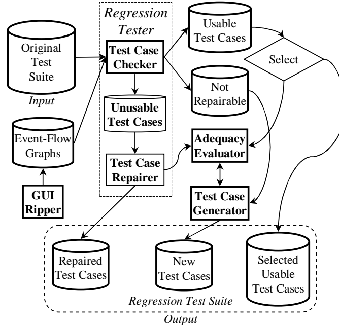
Fig. 4. Regression Tester's Components and their Interactions.
