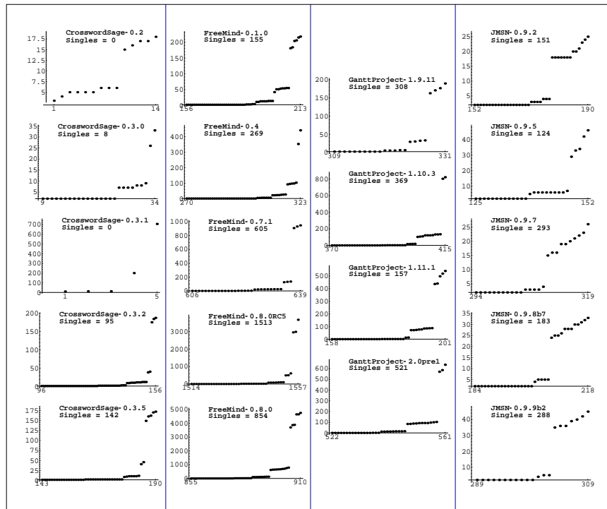
Fig. 12. Impact of Deleted EFG Edges on the Number of Unusable Test Cases.
