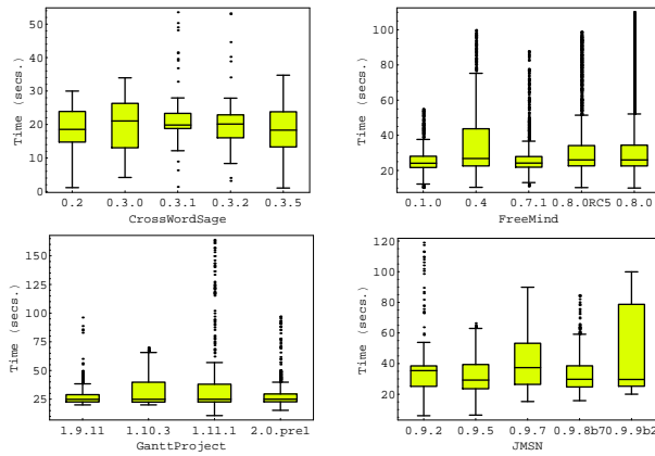
Fig. 17. Time Taken to Check Each Test Case Without Checker.
