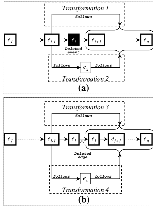
Fig. 3. Repairing an Event Sequence that Uses a (a) Deleted Event e_i , and (b) Deleted Edge (e_i, e_j) .
