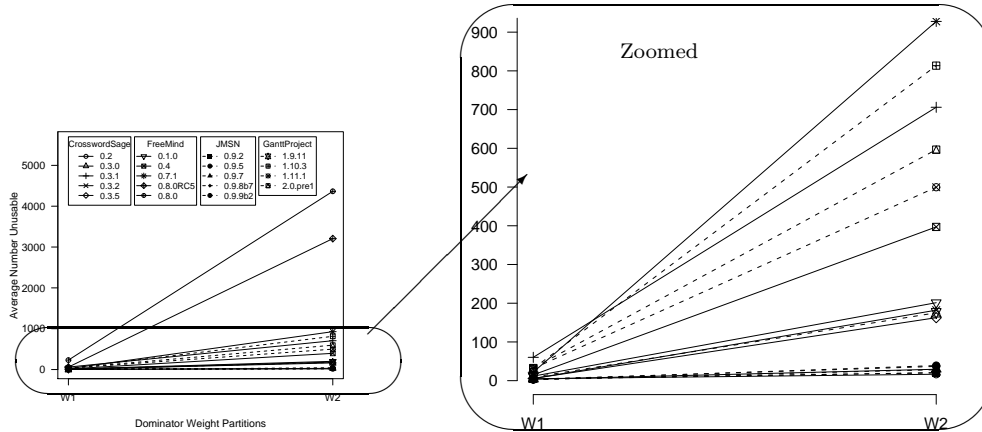
Fig. 15. Affect of Dominator Weight on Test Case Unusability
