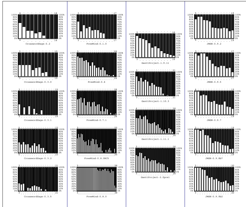
Fig. 10. Percentage of Test Cases that Remained Usable (unshaded part).
