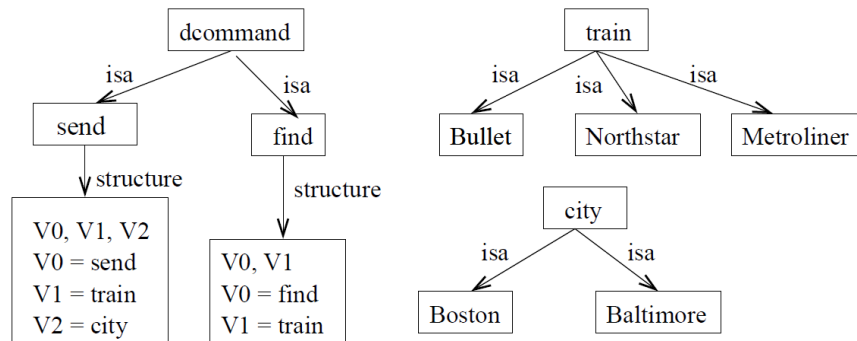
Figure 1.5: A fragment of ALFRED’s knowledge base prior to the user utterance “Send the Subway to Boston”.
