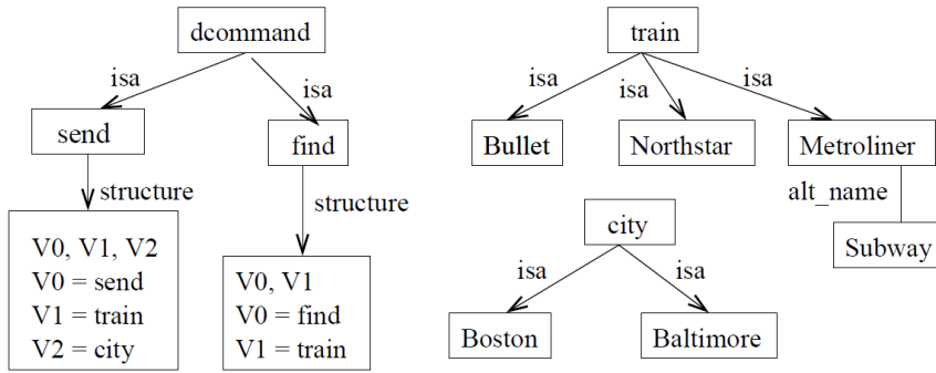
Figure 1.6: A fragment of ALFRED's knowledge base following the user utterance "Subway is Metroliner".
